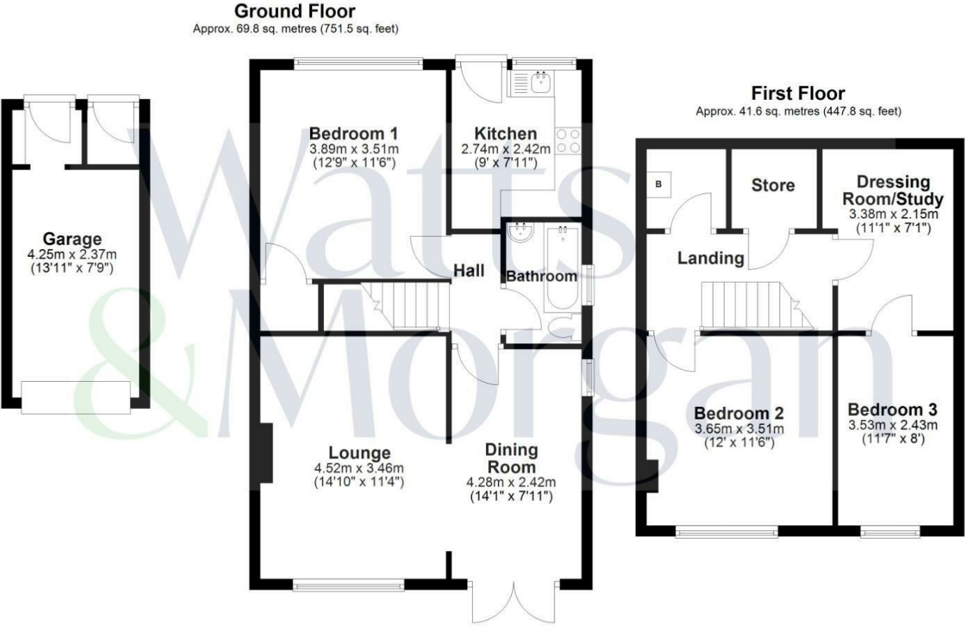
Total area: approx. 111.4 sq. metres (1199.2 sq. feet)
